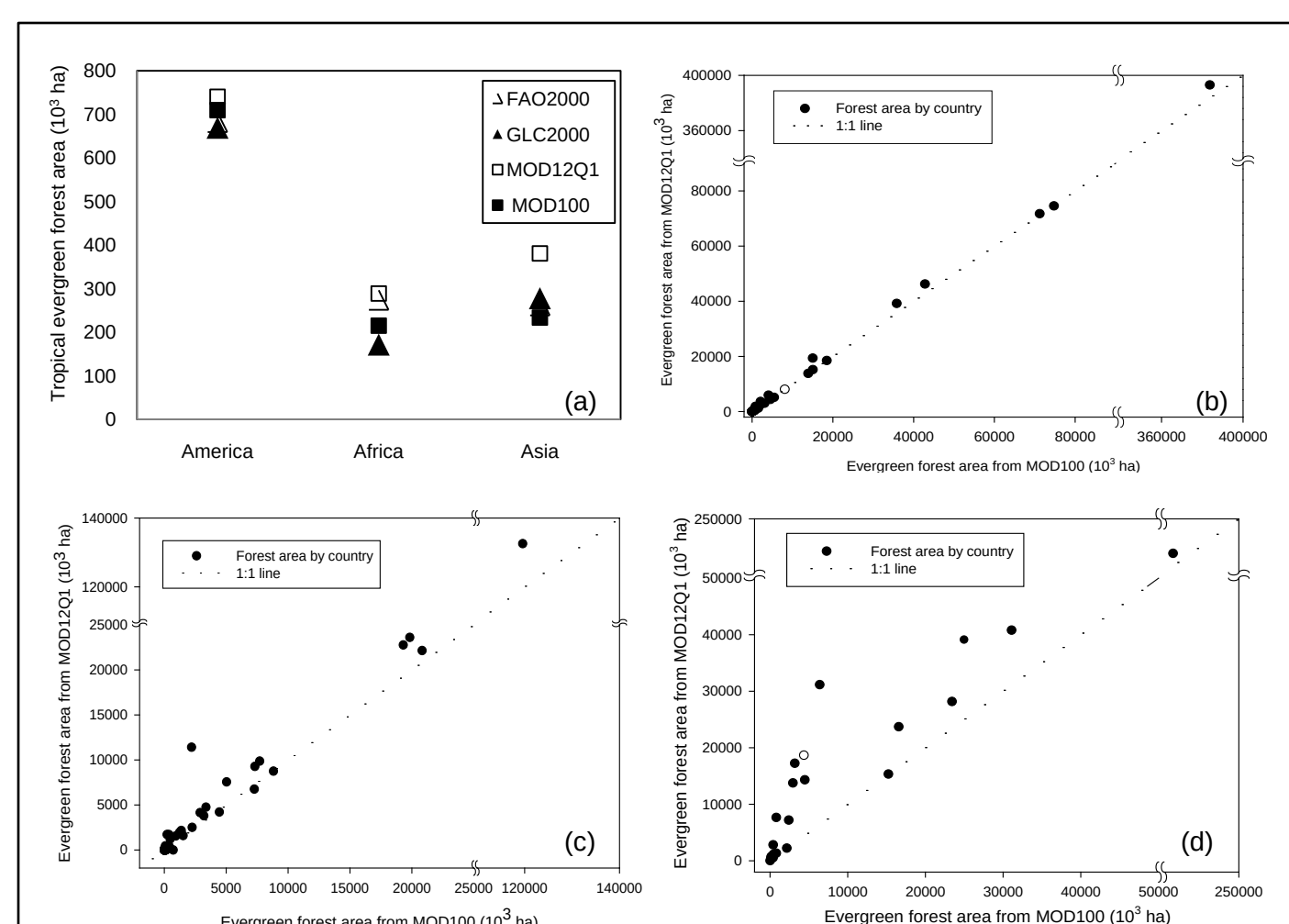
Fig. 2. A comparison of evergreen forest areas in the tropical America, Africa and Asia (30°N – 30°S); (a) among the four global forest datasets (MOD100, MOD12Q1, GLC2000 and FAO FRA2000); A country-level comparison for the area estimates of evergreen forests between the LSWI-based algorithm in this study (MOD100) and the standard MODIS Land Cover Product (MOD12Q1) in 2001 for (b) America; (c) Africa and (d) Asia.
