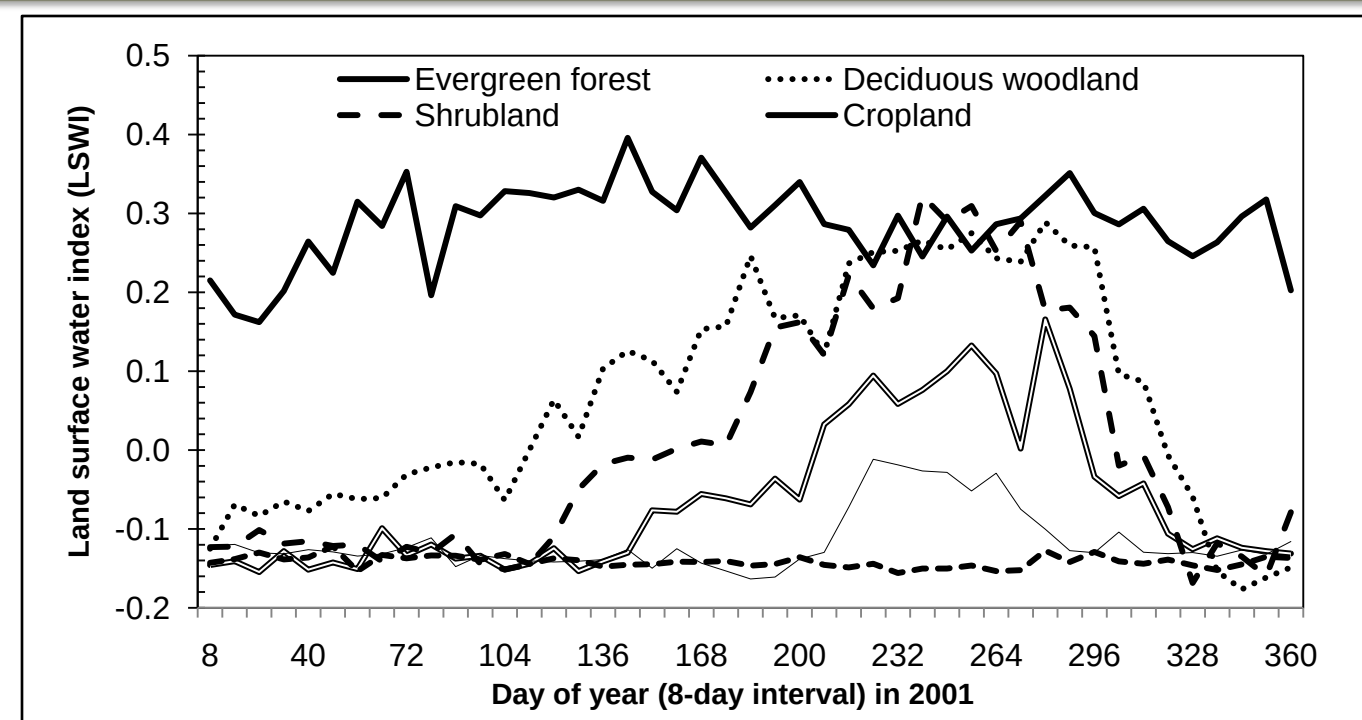
Fig. 1. The seasonal dynamics of Land Surface Water Index (LSWI) in 2001 from six sites that represent major land-cover types in the tropical Africa. The evergreen forest site (20.9086°E, 2.3042°S) was located at the Salonga national park of Democratic Republic of Congo (IUCN/WWF (1985)); the deciduous woodland site (3.8437°W, 9.4417°N) at the Comoé National Park of Côte d'Ivoire; the savanna shrubland site (2.4341°E, 11.7463°N) at the Benin National Park of Republic of Benin ( http://sea.unep-wcmc.org ); the cropland site (8.3158°E, 12.2098°N) in Nigeria (selected from an IKONOS image of November 7, 2000); the savanna grassland site (30.4783°E, 12.2829°N) at the CO2 flux tower site in Demokeya, Sudan ( http://www.fluxnet.ornl.gov/fluxnet ); and the desert site (28.2478°E, 18.2083°N) in Sudan.
